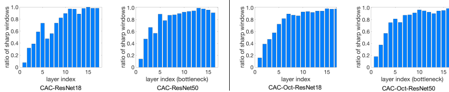
Figure 5: Visualization of the ratios of sharp windows for different layers in ResNet18 and ResNet50 on ImageNet. The layer index for ResNet50 denotes the index of the bottleneck block. We compute the ratios for different layers by averaging the samples in the validation set.
