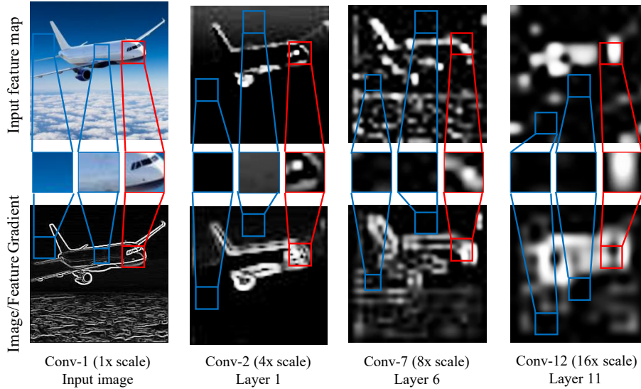
Figure 1: Demonstration of computational redundancy in the input feature maps of different layers of ResNet18 (pretrained on ImageNet). The top row and bottom row show the input feature maps and the corresponding gradient in different layers, respectively. Red boxes denote the sharp windows that contain the main content of the image. Blue boxes denote the smooth windows that contain limited information about the image and require redundant computation.
