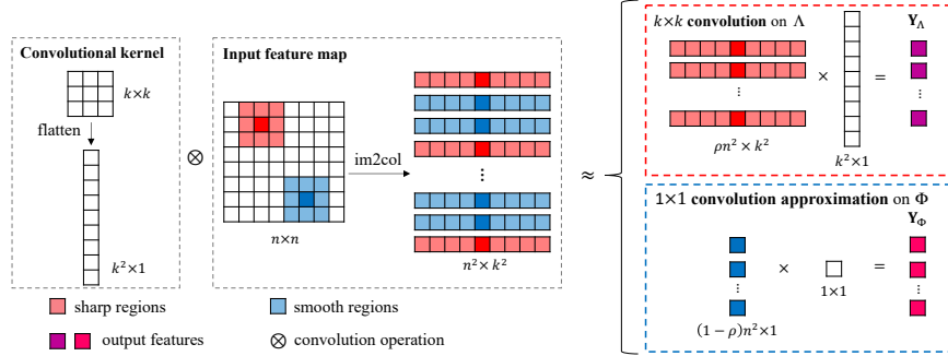
Figure 2: The computation method of Content-aware Convolution. We first divide the input feature maps into two parts, namely the sharp windows (red boxes) and smooth windows (blue boxes). Then, we perform k \times k convolution on sharp windows and 1 \times 1 convolution on smooth windows.
