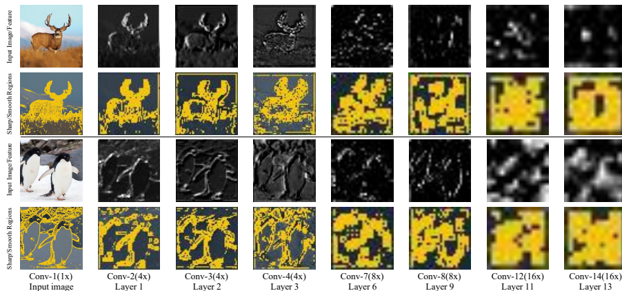
Figure 3: Visualization of the feature maps of different layers in CAC-ResNet18 on ImageNet. For each image, the top row shows the feature map of different layers and the bottom row shows the corresponding map of sharp windows detected by CAC. In the bottom row, yellow regions denote the sharp windows to perform 3 \times 3 convolution and the dark regions denote the smooth ones to perform 1 \times 1 convolution. We scale the feature maps of different layers to the same spatial size for better visualization.
