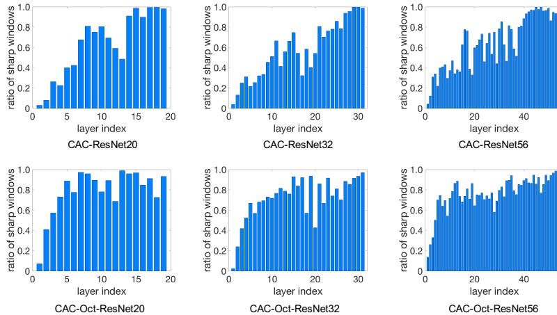
Figure 4: Visualization of the ratios of sharp windows for different layers in ResNet20, ResNet32, and ResNet56 on CIFAR-10. We compute the ratios by averaging the ratios over 10,000 testing samples.
