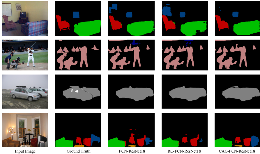
Figure 6: Visual comparison of the segmentation masks produced by different methods. The first and the second columns show the input images and the corresponding ground truth segmentation masks, respectively. The last three columns show the segmentation masks predicted by different models.
